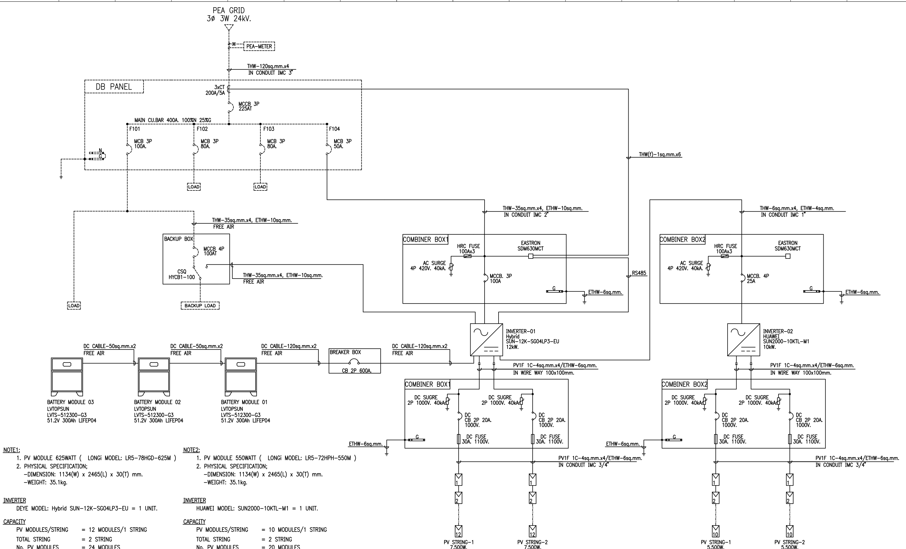
Solar Cell System Single Line Diagram SCALE NONE
